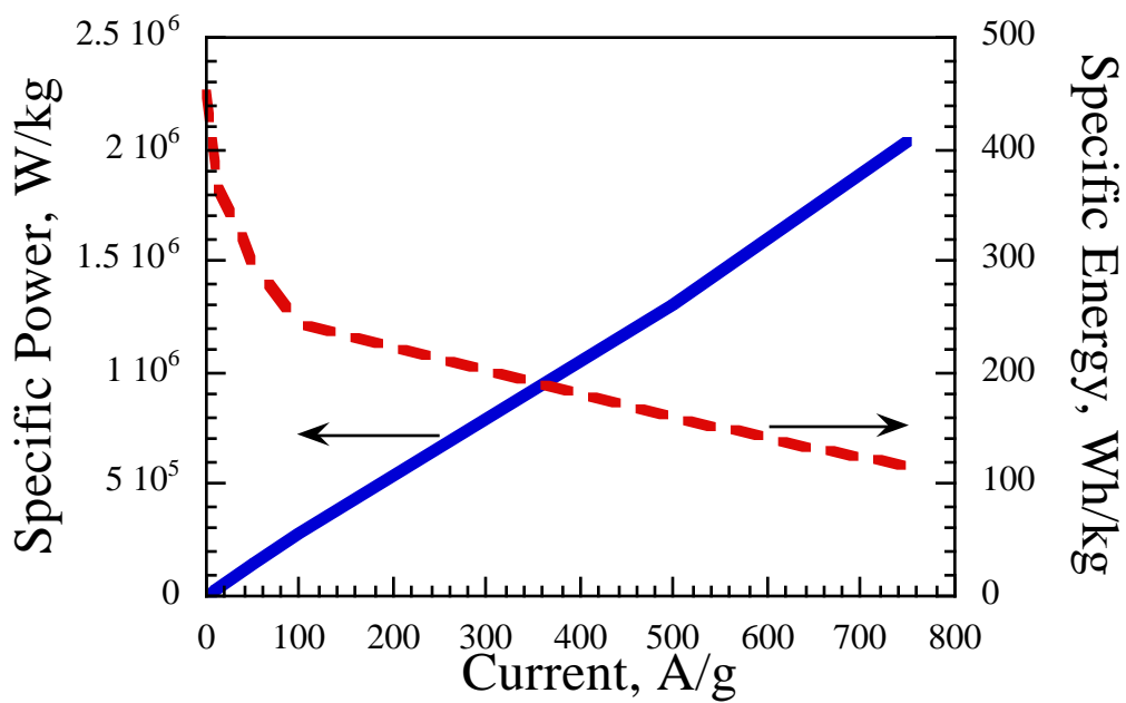
Specific energy and power of a V_2O_5 ARG/ Nickel composite electrode measured under galvanostatic conditions. All values are based on mass of active material ( V_2O_5 ).
