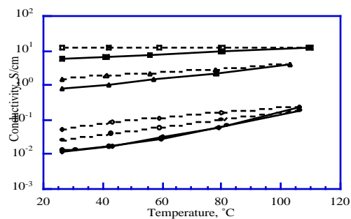
Electronic conductivity of V 2 O 5 (circles), Ag 0.01 V 2 O 5 (diamonds), Ag 0.1 V 2 O 5 (triangles), AgV 2 O 5 (squares) xerogel dip-coated samples as a function of temperature. Data taken in the heating cycle are indicated by full dots. Empty dots are used for the cooling cycle.
