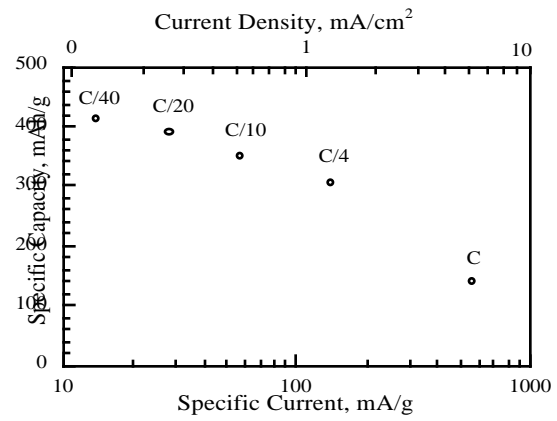
Figure 1. Hex.V 2 O 5 composite electrode specific capacity (mAh/g) versus specific current. The discharge rates and the current densities are also indicated in the figure.
